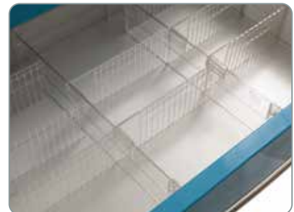
Set of dividers on first 3 drawers
